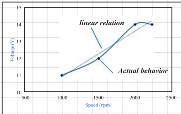
Fig. 6. Relationship between Voltage and rotation
